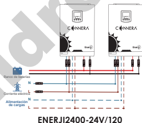
ENERJI2400-24V/120
